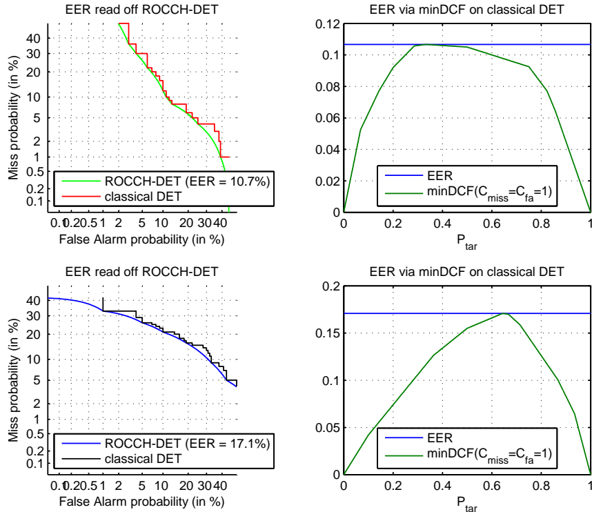
Figure 4: Two examples of ROCCH-DET vs classical stepy DET. The equality of ROCCH-EER and max minDCF is demonstrated. (Here \tilde{\pi} = P_{tar} ).
